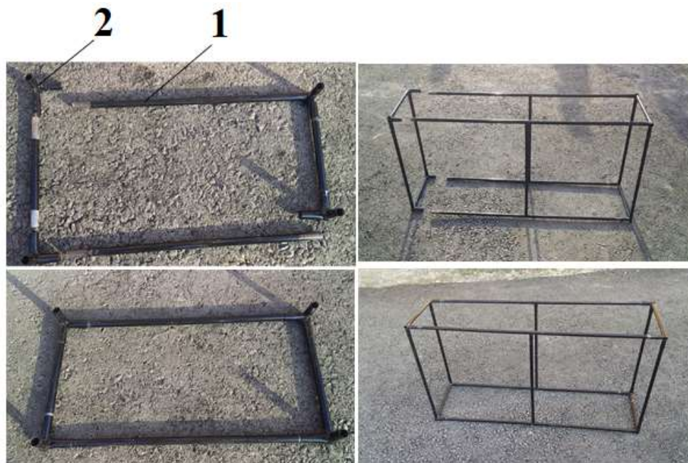
Figure 1. Fragments of assembled parts of the frame of a newly created device for receiving, transporting and storing live cocoons
