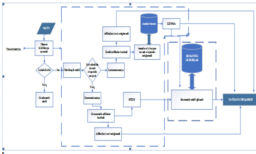
2-rasm. Alisher Navoiy mualliflik korpusida ish jarayoni quyidagi biznes-jarayon modeli.
