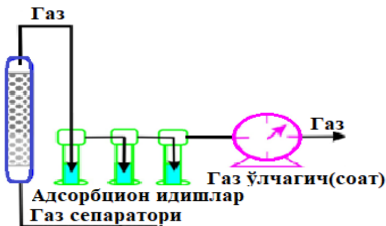
5-rasm. Neft yo'ldosh gazlarini vodorod sulfiddan tozalash uchun eksperimental adsorber qurilmasi
