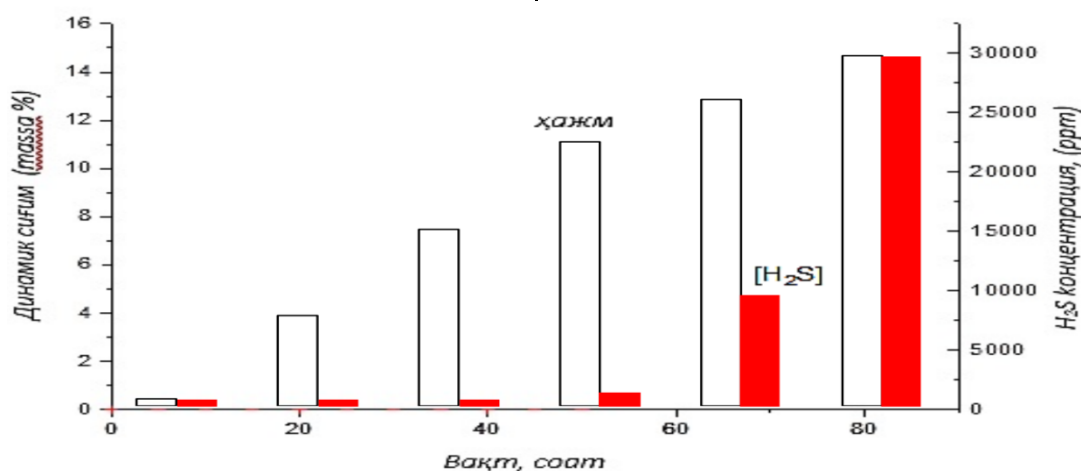
6-rasm. Gazlarni vodorod sulfiddan tozalashda vaqt davomida adsorberdan chiqishda \text{CaCl}_2 \cdot \text{ZnCl}_2 \cdot \text{MnCl}_2 / \text{YUKS} xemosorbenti dinamik sig'imining o'zgarishi.
