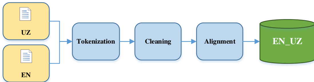
Figure 4. Sentence matching sequence based on heuristic algorithm.
